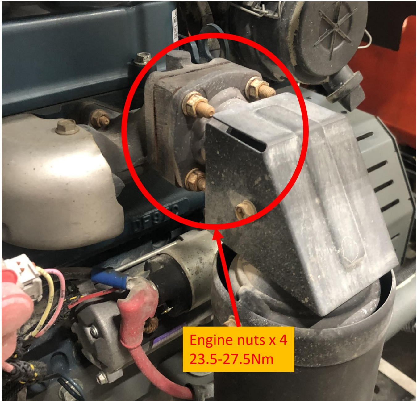
Fig. 1: Torque values for 33K models equipped with WG 972 engine.
