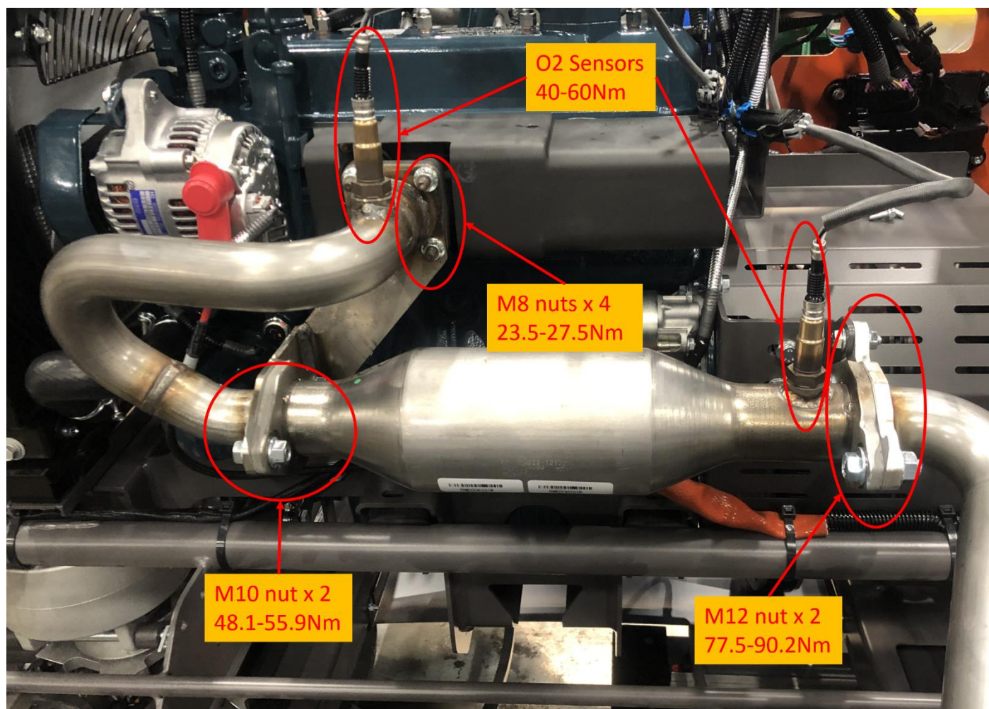
Fig. 2: Torque values for 57K models equipped with WG 1605 engine.
