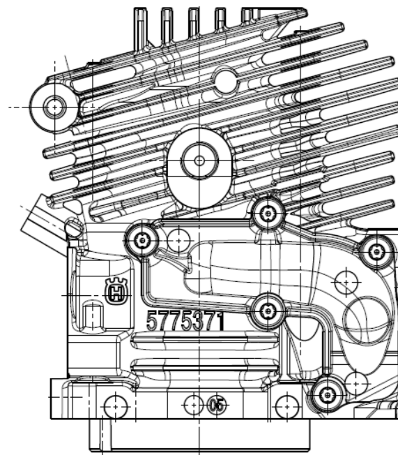
581476105 Cylinder Assy K 770 II
