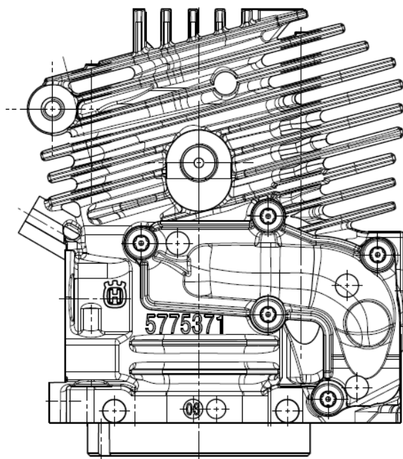
581476104 Cylinder Assy K 770
